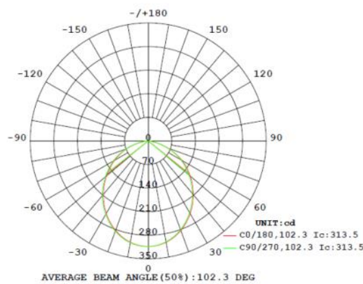
Luminous Intensity Distribution Diagram Set at 5000K
