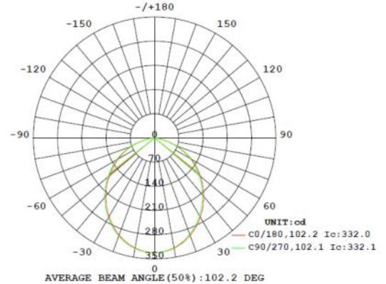
Luminous Intensity Distribution Diagram Set at 4000K
