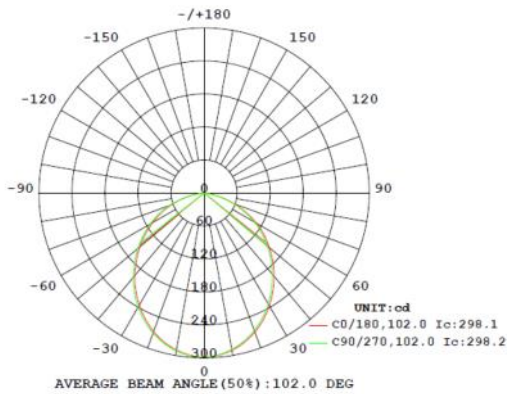
Luminous Intensity Distribution Diagram Set at 3000K
